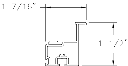
LIFT RAIL (4006) EXTRUDED RIGID PVC
