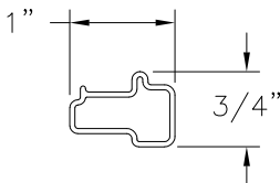
LOCK RAIL/ STILE REINFORCEMENT (204-B) ALUMINUM 6063-T5
